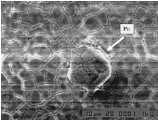
Fig. 6. SEM micrograph of the laser treated surface after 30 min of electrochemical polarization at 2.7 V showing pit initiation.
