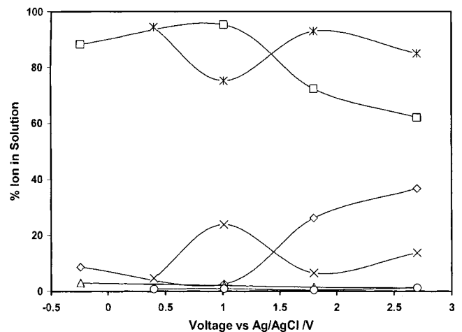
Fig. 3. Plot of percentage Ti, Al, V of the untreated and laser treated specimen from ICP after electrolysis at selected potentials for 2 h. Untreated: ( \diamond ) Ti, ( \square ) Al, ( \triangle ) V; treated: ( \times ) Ti, ( * ) Al, ( \circ ) V.
