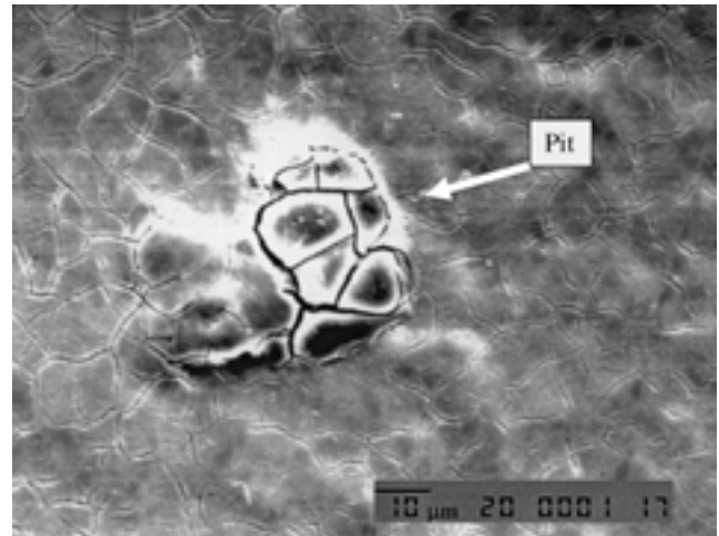
Fig. 7. SEM micrograph of the laser treated surface after 120 min of electrochemical polarization at 2.7 V showing pit site formation.
