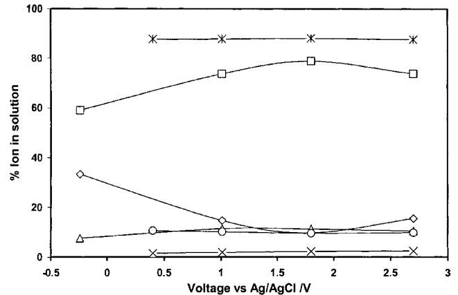
Fig. 2. Plot of percentage Ti, Al, V of the untreated and laser treated specimen from ICP after electrolysis for 30 min at selected potentials. Untreated: ( \diamond ) Ti, ( \square ) Al, ( \triangle ) V; treated: ( \times ) Ti, ( * ) Al, ( \circ ) V.
